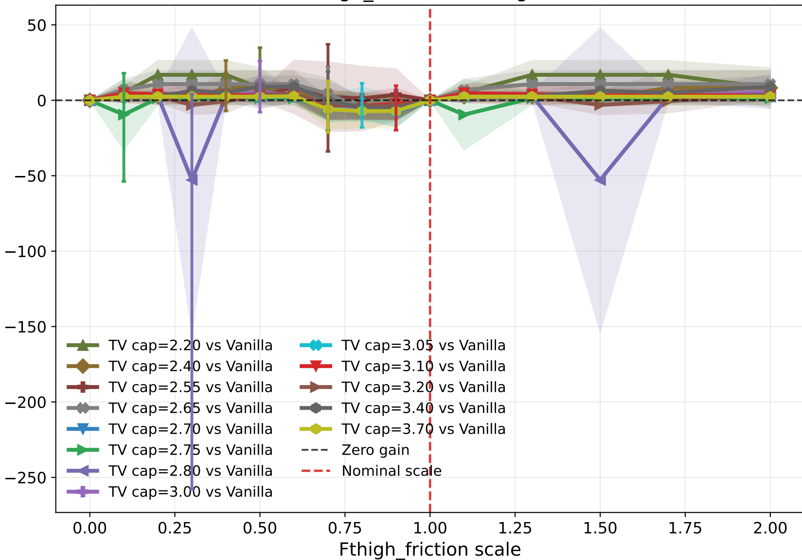
Fthigh_friction robust gain
